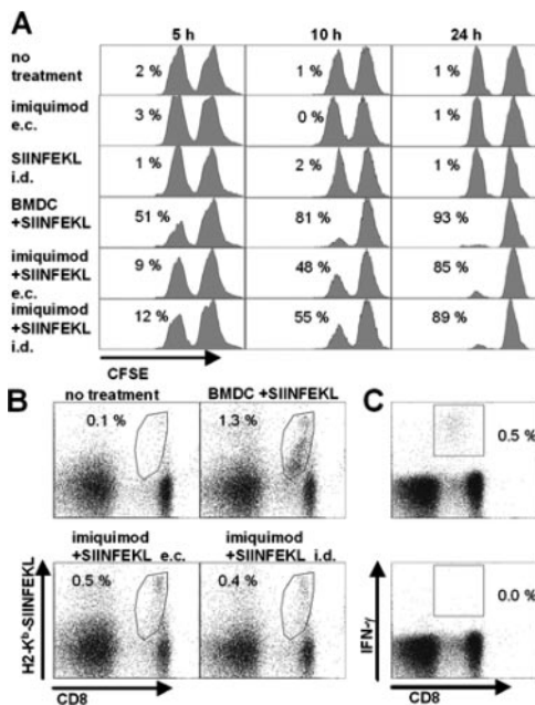
FIGURE 4. Transcutaneous peptide immunization of wild-type mice with imiquimod elicits a potent CTL response in vivo. A , C57BL/6 mice were treated with TCI using imiquimod ointment (50 mg) or peptide (SIINFEKL, 150 \mu g) separately or in combination twice daily on 2 consecutive days. After 8 days in vivo, cytolytic activity against SIINFEKL (1 \mu M)-loaded CFSE low or non-peptide-loaded CFSE high syngenic splenocytes was evaluated after 5–24 h. The depicted numbers correspond to the percentage of specific lysis. B , Splenocytes from treated mice were stained for peptide-specific CD8 + T cells using a SIINFEKL-loaded recombinant dimeric H2-K b -mIgG1 fusion protein to detect peptide-specific CD8 + T cells. The depicted numbers represent the percentage of cells in the indicated region. C , Splenocytes from imiquimod + SIINFEKL e.c.-treated mice were stimulated for 6 h in the presence ( upper panel ) or absence ( lower panel ) of SIINFEKL (50 nM), adding brefeldin A for the last 4 h of incubation. The production of IFN- \gamma ex vivo was then analyzed by intracellular staining for IFN- \gamma . The numbers shown indicate the percentage of cells in the indicated region. All depicted results are representative of three independent experiments using two mice per group.
