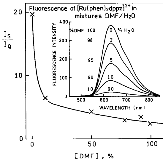
FIG. 16. Enhancement of [Ru(bpy)_2(dppz)]^{2+} on silver island films in water-DMF mixtures.
