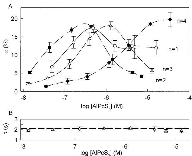
FIGURE 2 (A) The dependence of the relative amplitude of gramicidin photoinactivation ( \alpha , mean \pm SE, %) on the concentration of phthalocyanines with different numbers of sulfonate groups ( n ). Phthalocyanines with n = 2-4 are added from aqueous solutions, while \text{AlPcS}_1 is dissolved in 1:1 methanol and 0.1 M NaOH. The initial value of the current ( I_0 ) is \sim 1.0 \mu\text{A} . (B) The dependence of the characteristic time of photoinactivation ( \tau , mean \pm SE) on the \text{AlPcS}_3 concentration.
