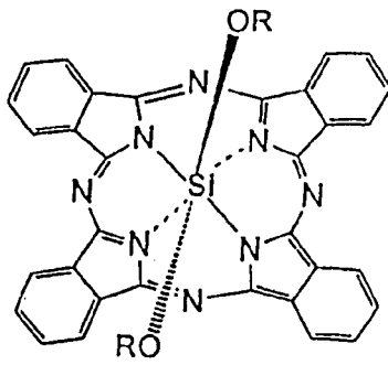
Silicon Phthalocyanine
