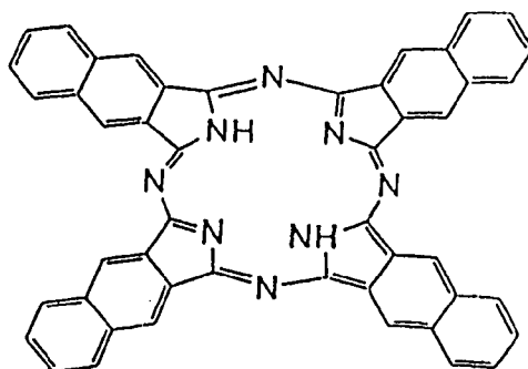
Naphthalocyanine
