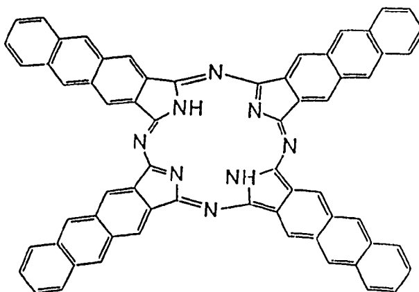
Anthranylocyanine
