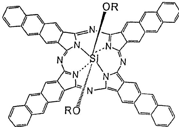
Silicon Anthracyanine
