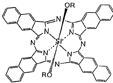
Silicon Naphthalocyanine
