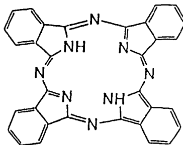
Phthalocyanine
